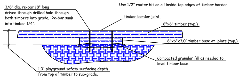
Playground Border Detail - 6"x6" timbers
