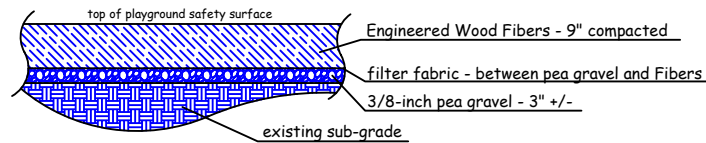
Safety Surfacing Installation
